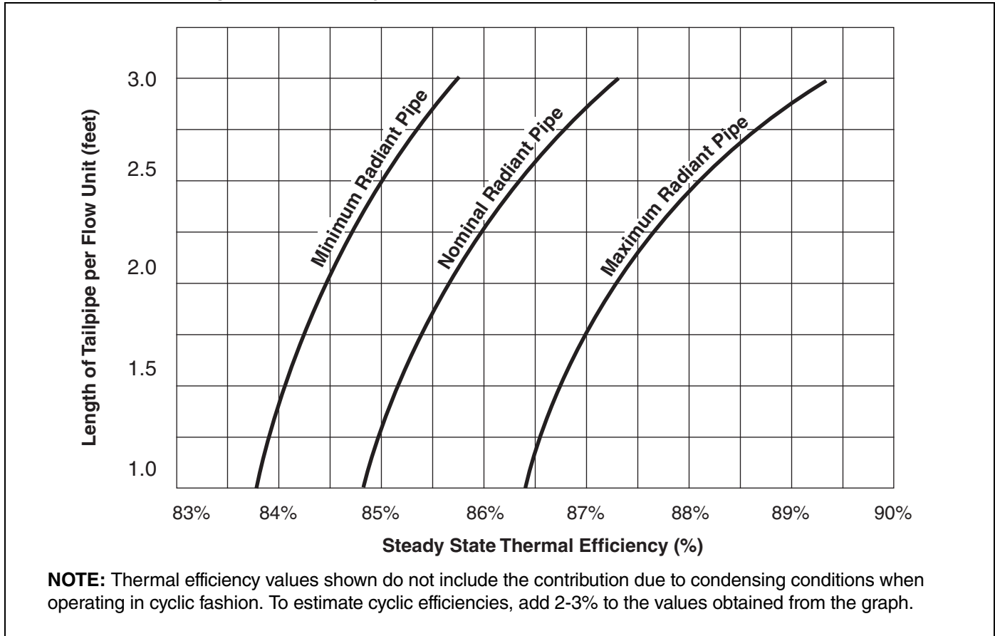
FIGURE 16: Tube Length vs. Efficiency
