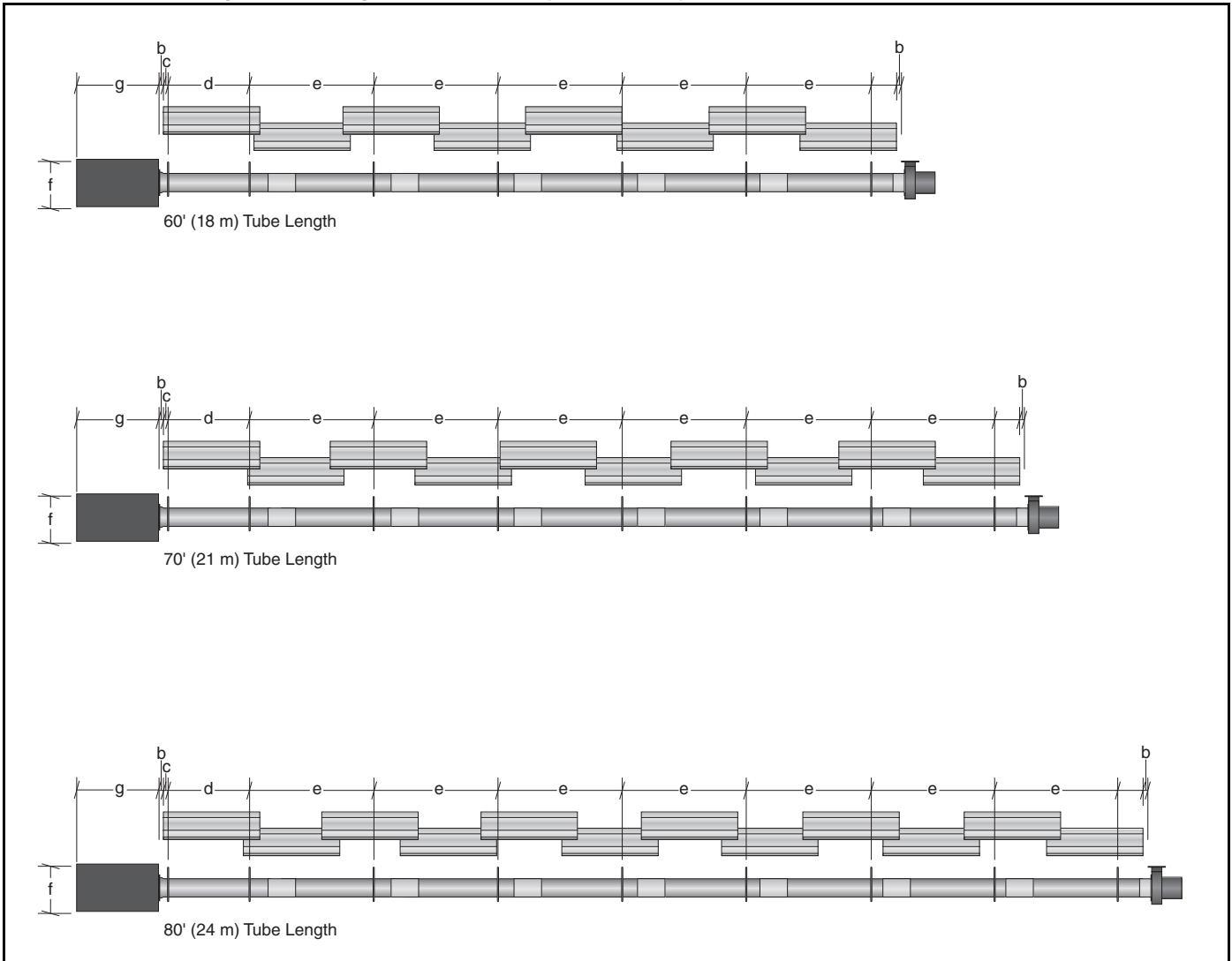
FIGURE 17: Unitary Linear Layout Overview (Continued)
