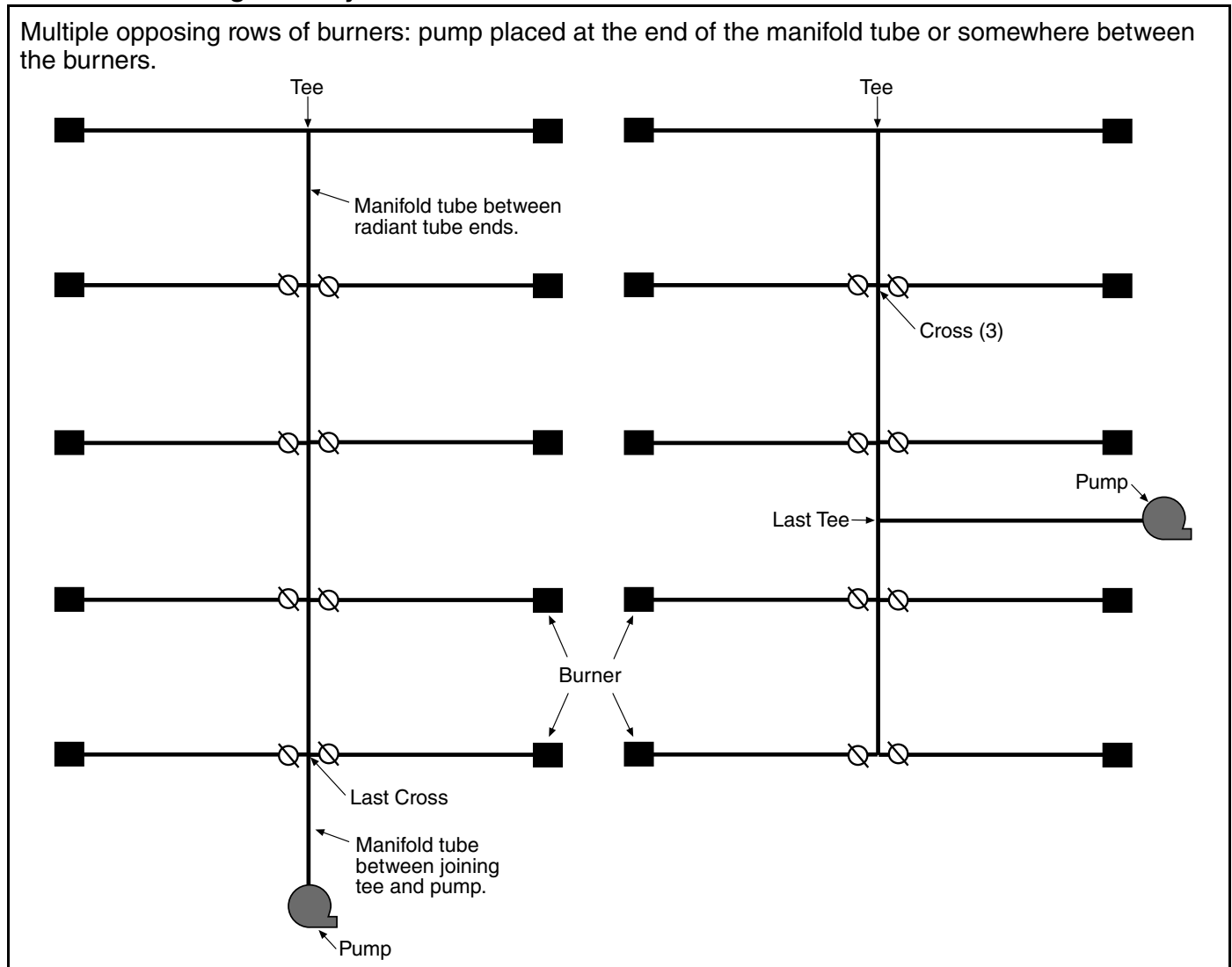
FIGURE 25: Herringbone Layout
