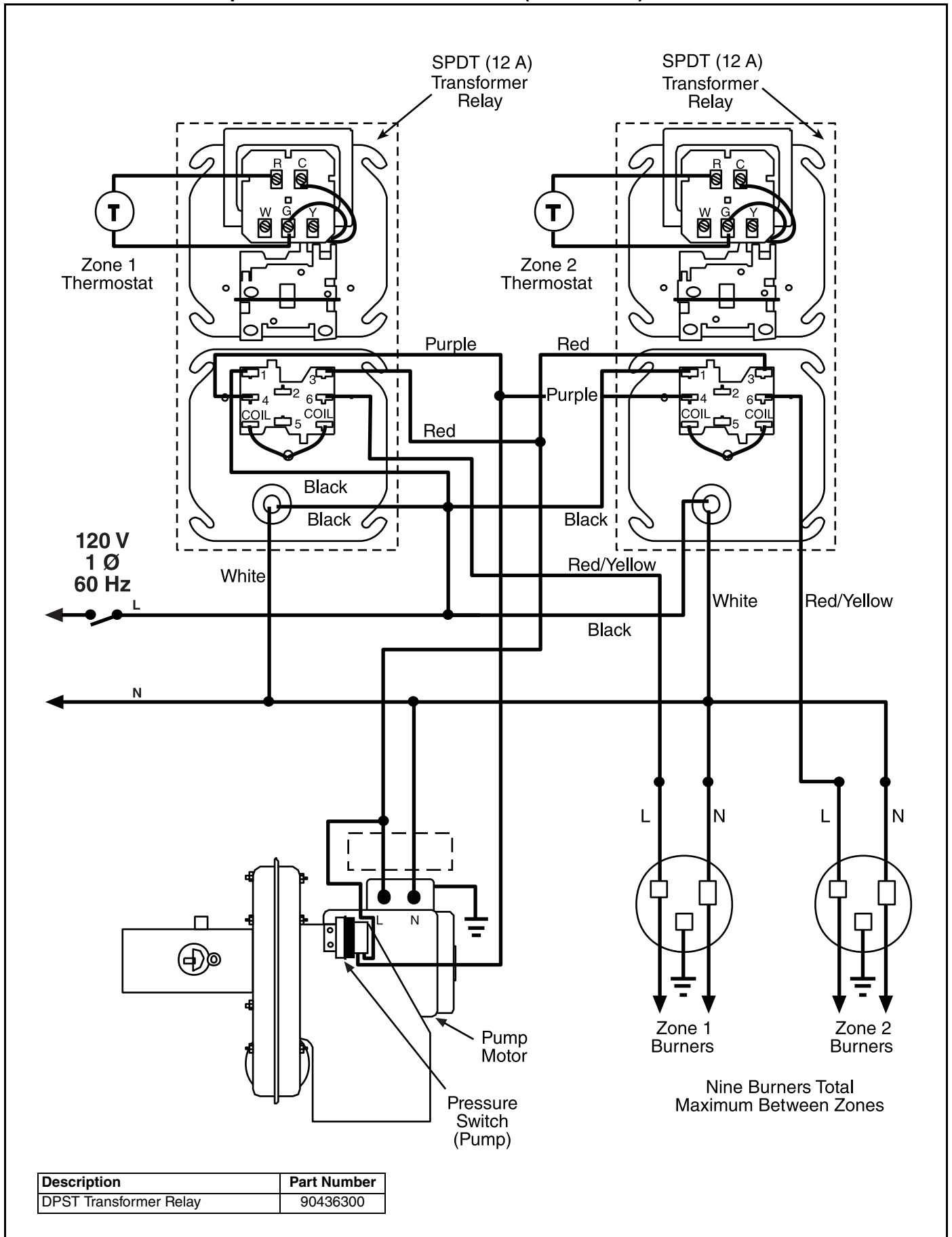
FIGURE 33: Two Zone Operation without Control Panel (Multiburner)
