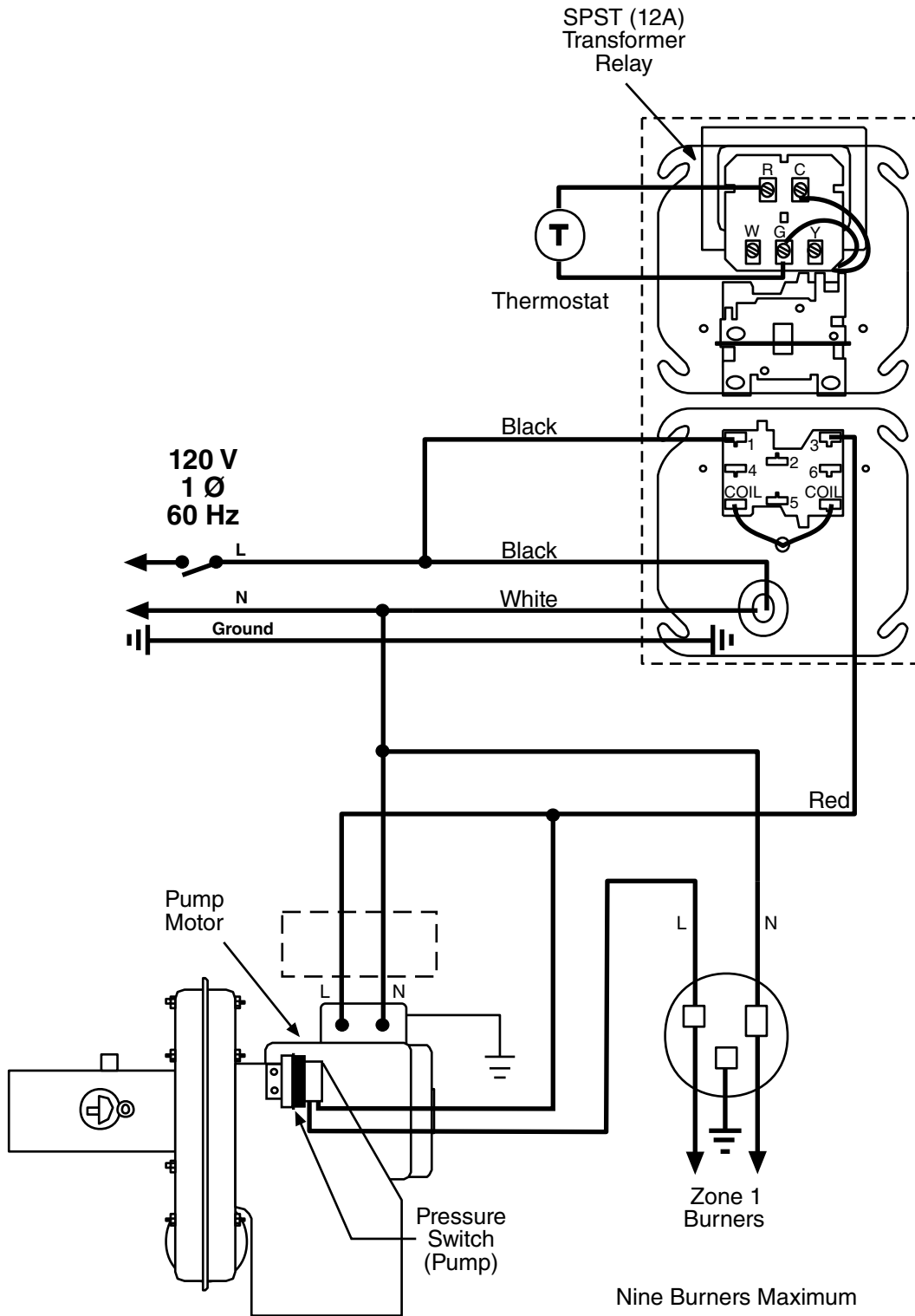
FIGURE 32: One Zone Operation without Control Panel (Multiburner)
