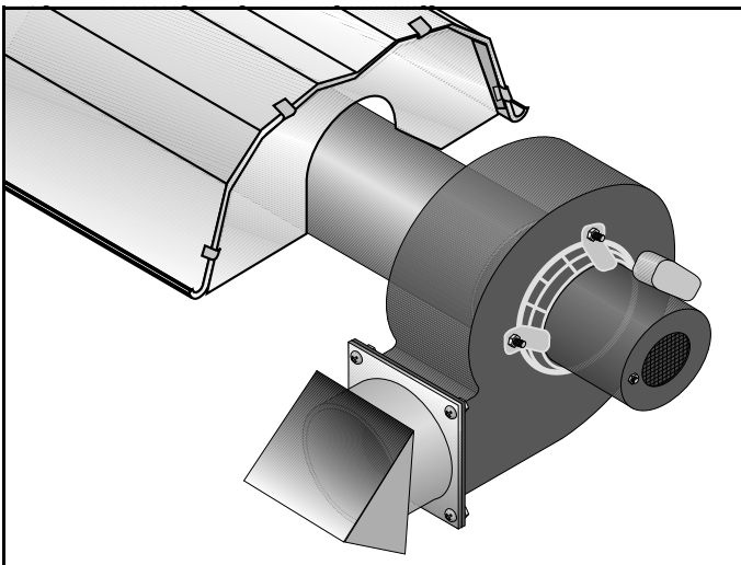
FIGURE 27: Fan Termination
