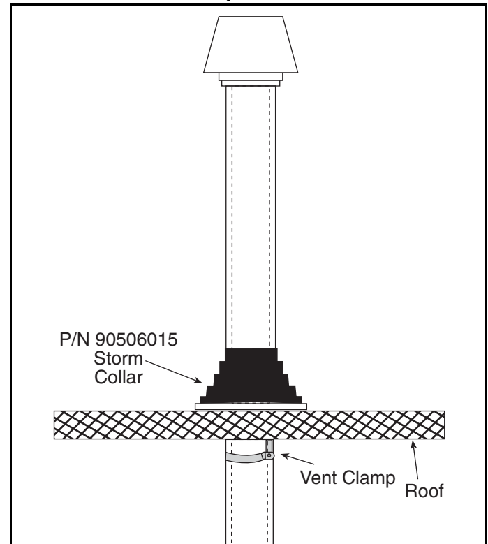
FIGURE 31: Vent Clamp
