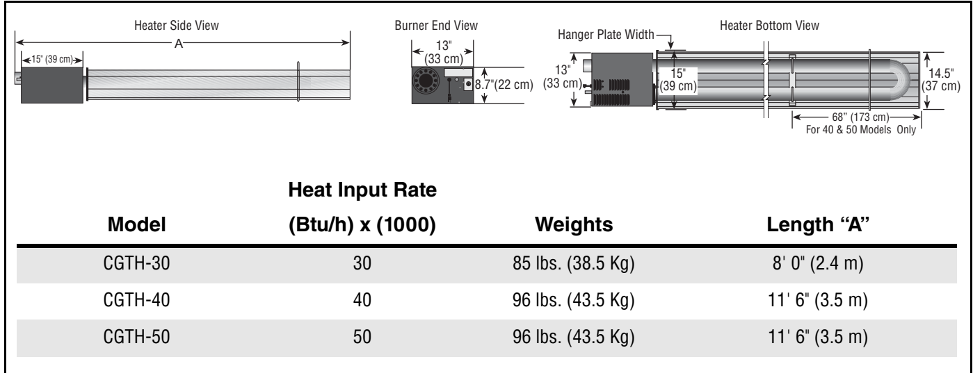
FIGURE 4: Specifications
