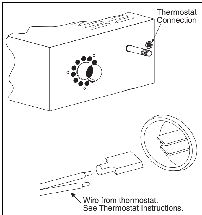
FIGURE 33: Thermostat Installation Rear View
