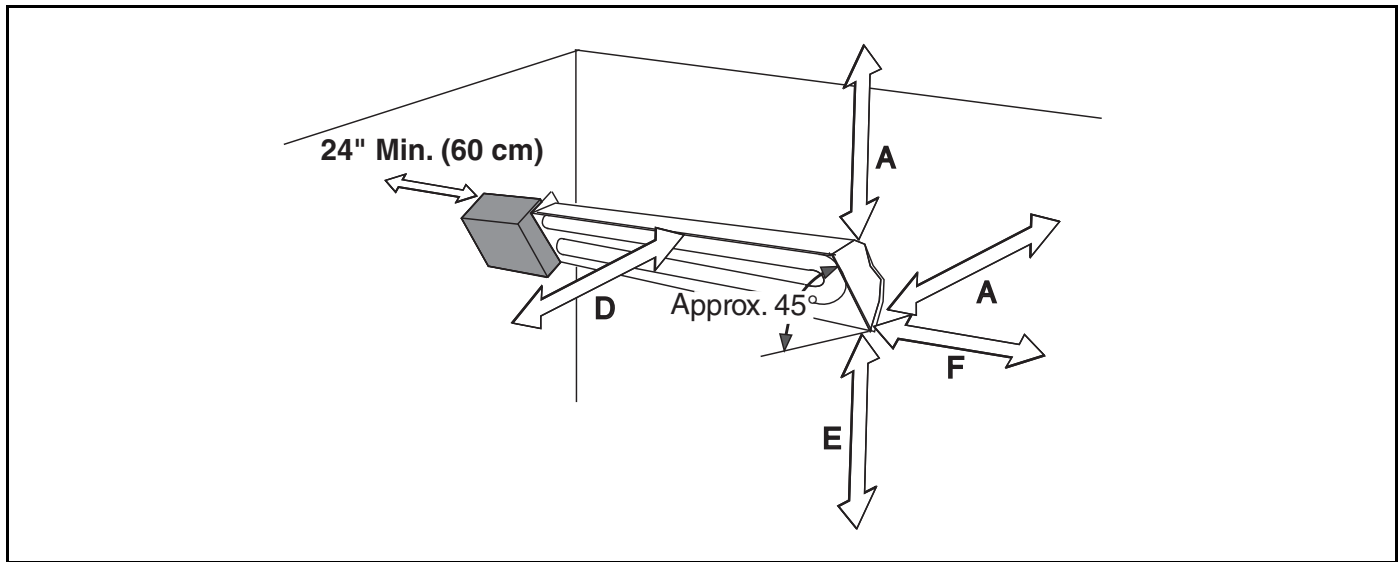
FIGURE 7: 45° Tilted Installations
