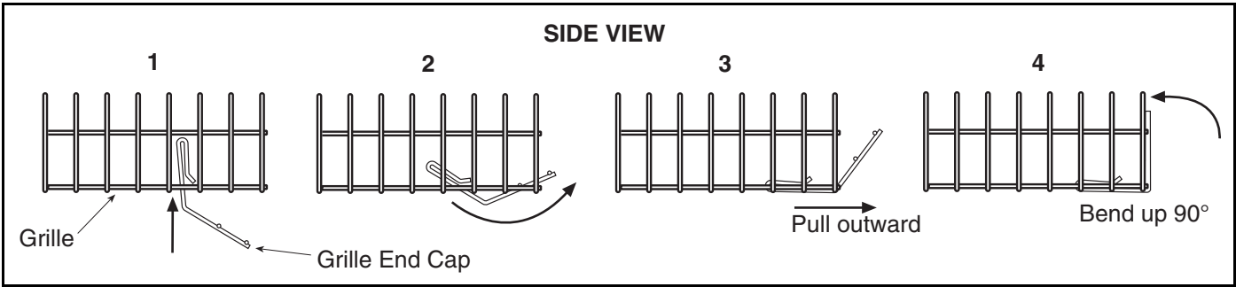
FIGURE 16: Grille End Cap Installation
