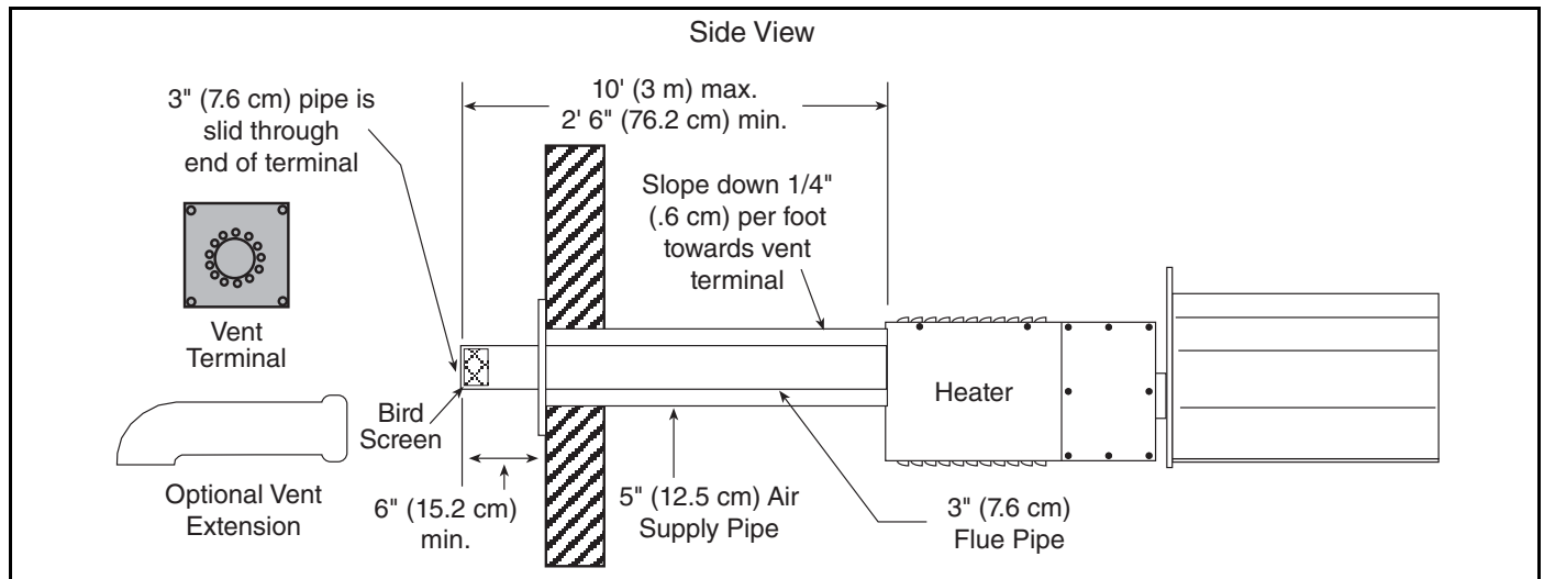
FIGURE 19: Horizontal Installation Side View
