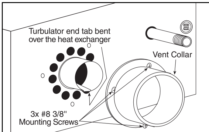
FIGURE 18: Rear View
