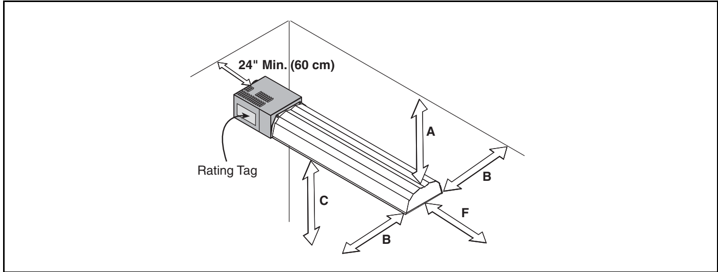
FIGURE 7: 45° Tilted Installations
