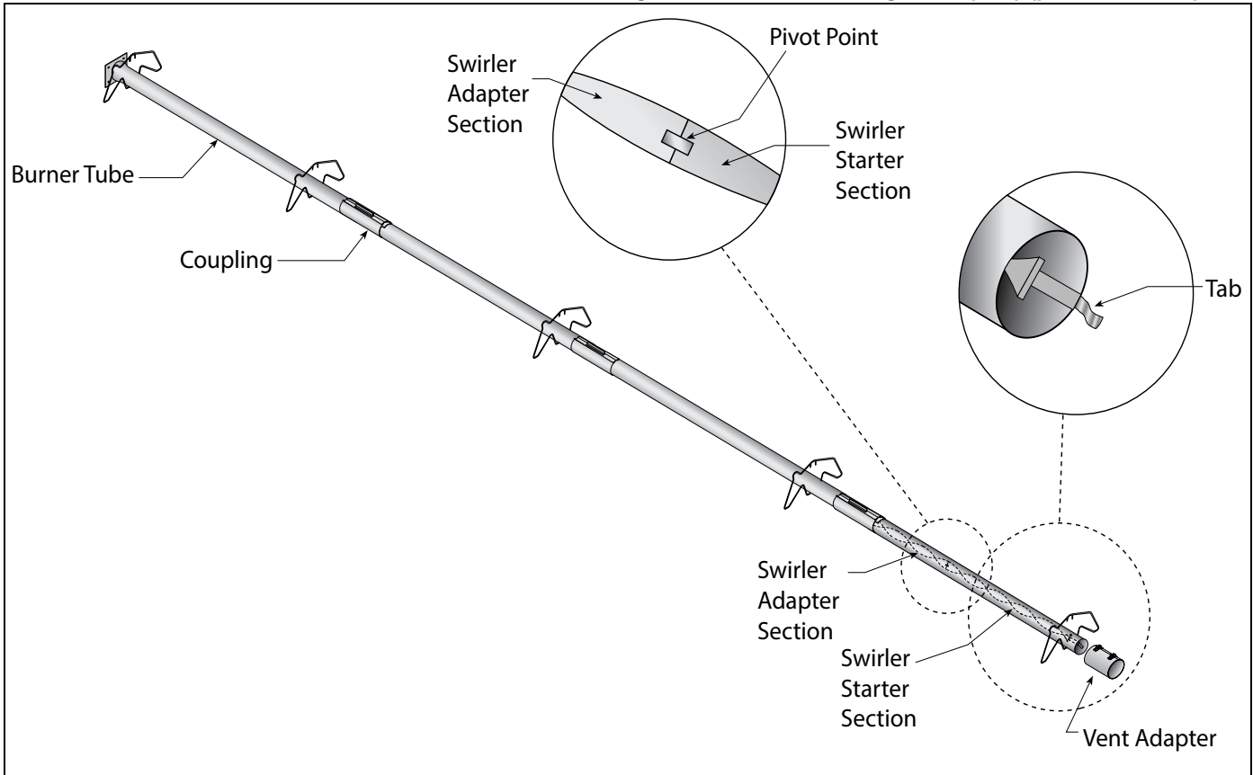
FIGURE 23: Swirler Installation Model: CTH2V-150, 40' U-Tube; Swirler Package - 10' (3 m) (p/n 03051509K)
