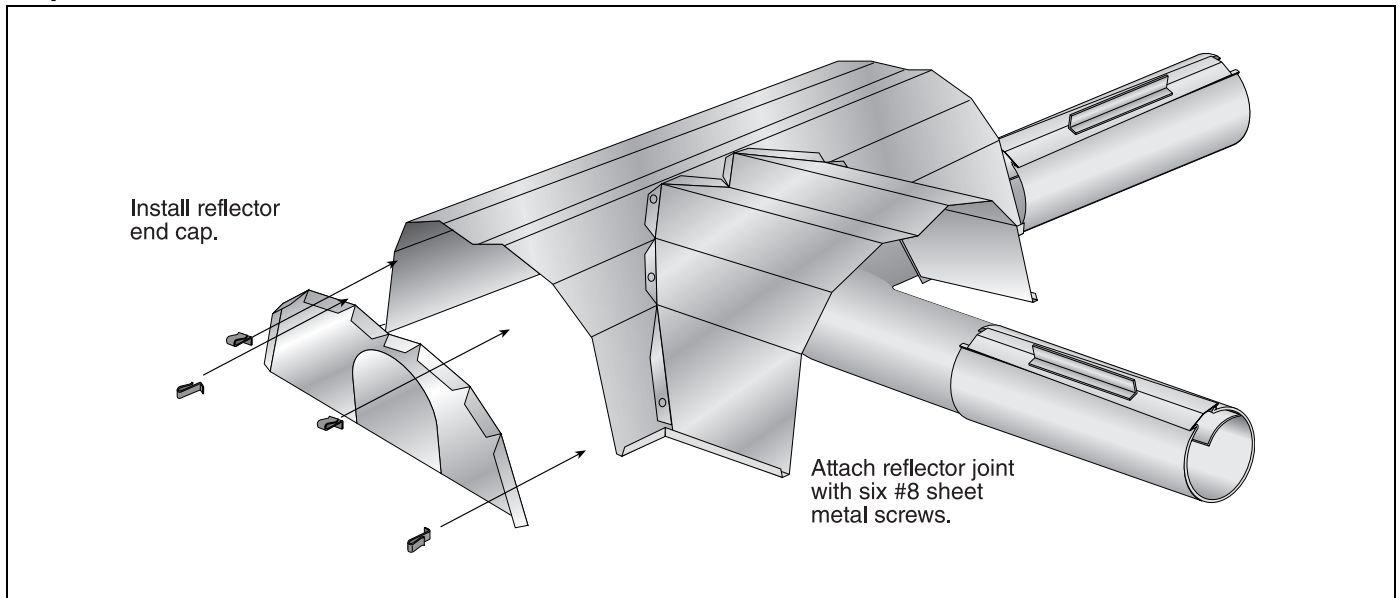
FIGURE 30: Reflector Joint Detail
