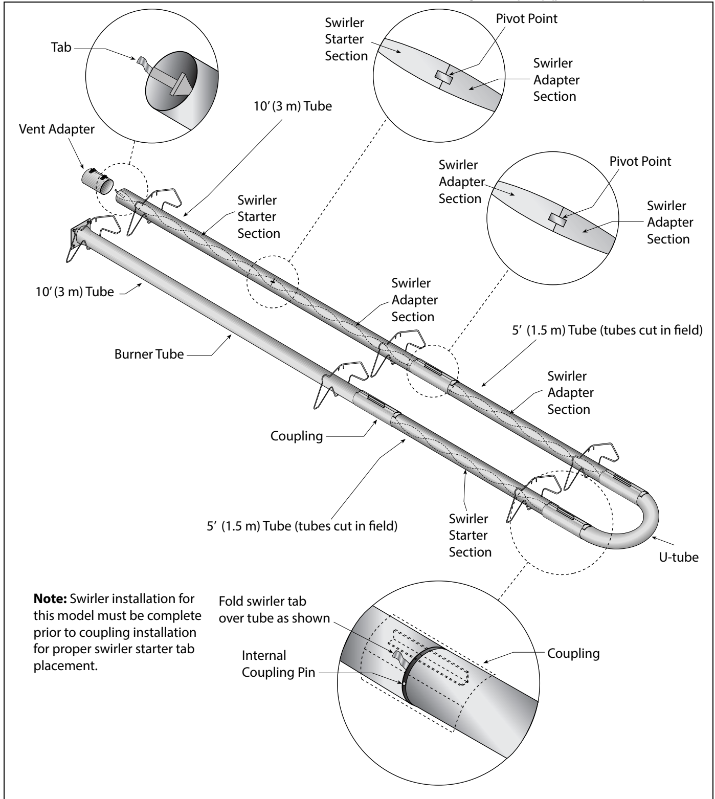
FIGURE 21: Swirler Installation Model: CTH2V-125, 30' U-Tube; Swirler Package - 20' (6 m) (p/n 03051511K)
