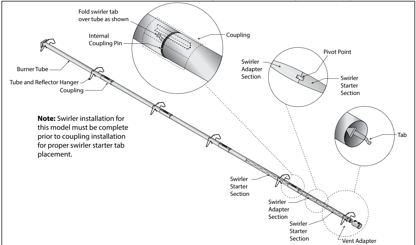
FIGURE 25: Swirler Installation Model: CTH2V-175, 50' Even U-Tube; Swirler Package - 15' (4.5 m) (p/n 03051510K)
