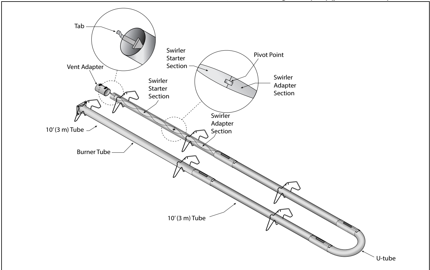
FIGURE 23: Swirler Installation Model: CTH2V-150, 40' U-Tube; Swirler Package - 10' (3 m) (p/n 03051509K)
