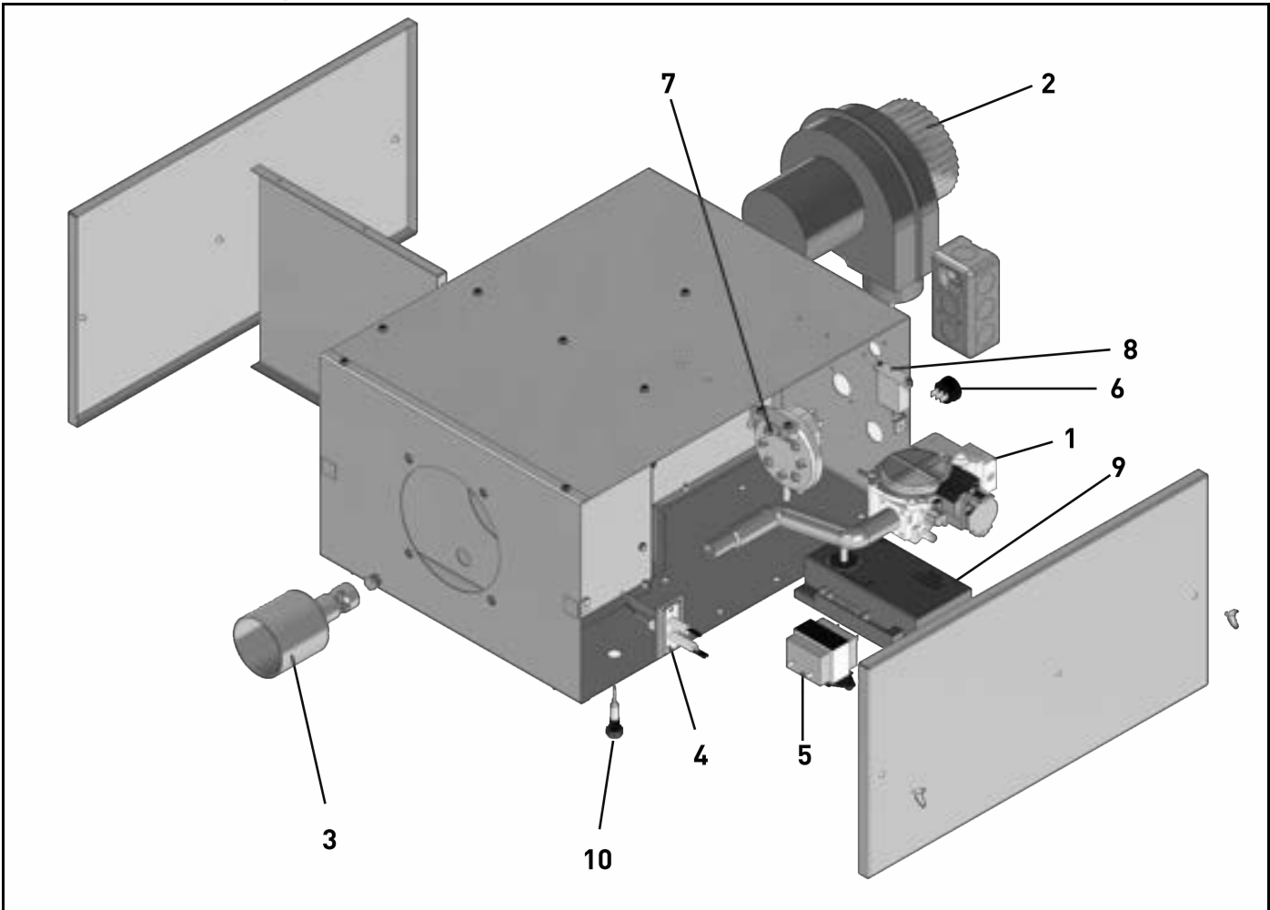
FIGURE 33: Burner Exploded View
