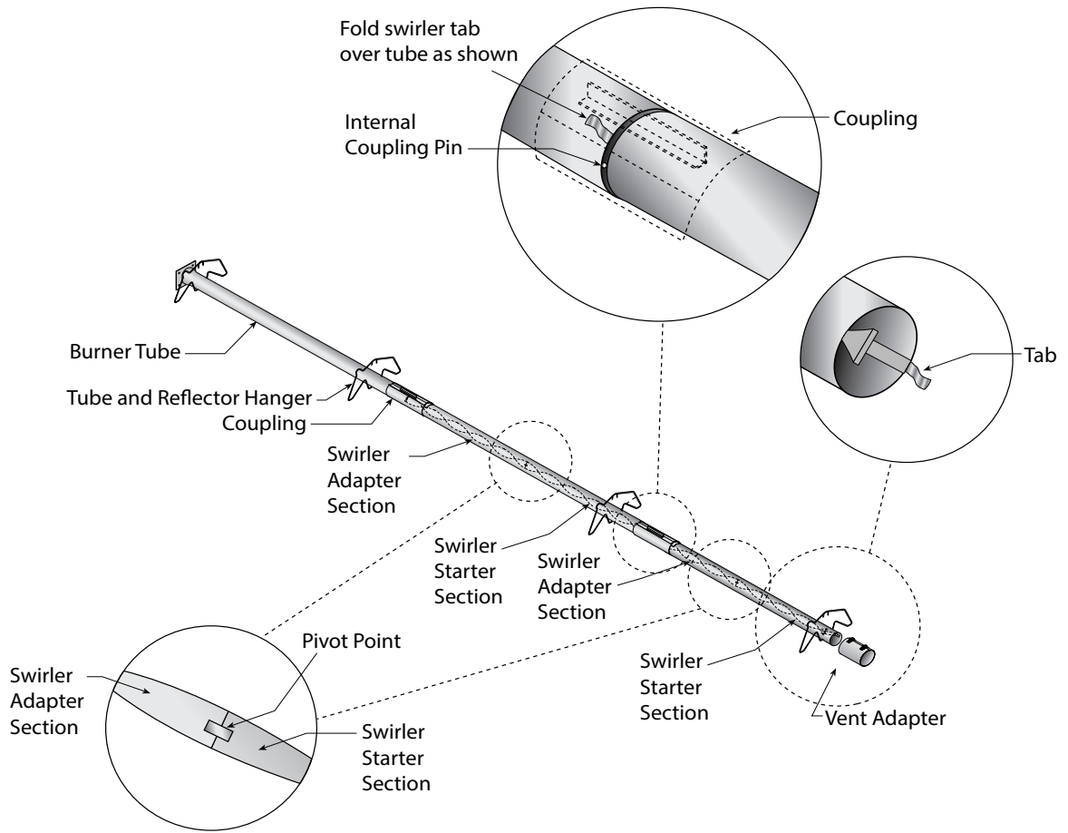
FIGURE 20: Swirler Installation Model: CTH2V-125, 30' Straight Tube; Swirler Package - 20' (6 m) (p/n 03051511K)
