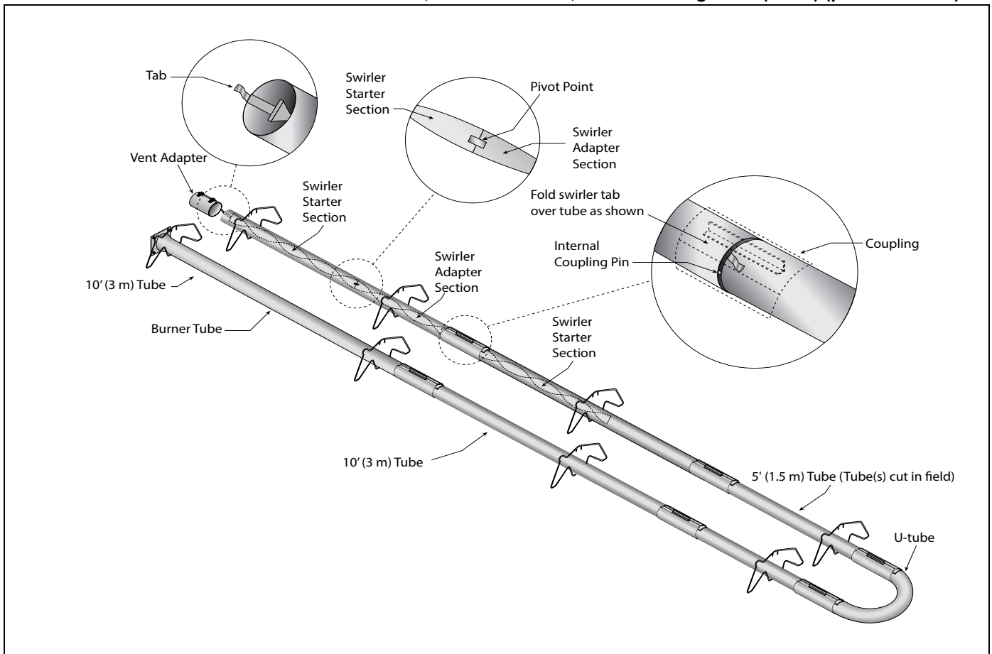
FIGURE 25: Swirler Installation Model: CTH2V-175, 50' Even U-Tube; Swirler Package - 15' (4.5 m) (p/n 03051510K)
