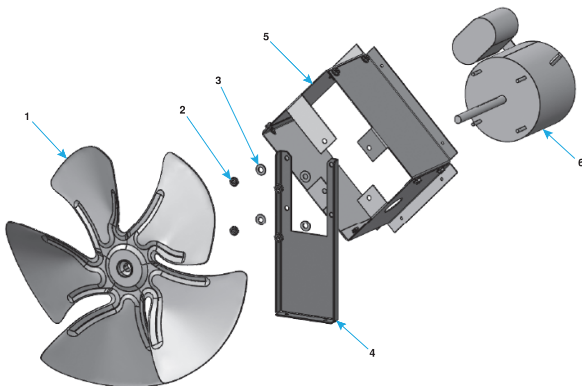
Figure 4. Fan and Motor Assembly (Refer to Table 4 )
